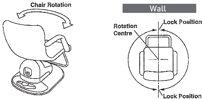
Fig.4-3 Chair Rotation
