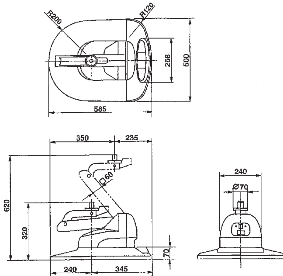
Fig.2-1 Dimensions
