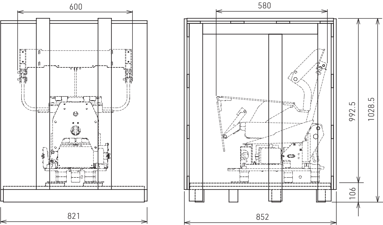
<SUITE / NOBLE Seat body: Movable legrest type> Basin body 48 kg, Wood frame 30 kg
